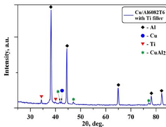
Fig. 7. X-ray patterns of the welded specimen, with Ti filler [12]
